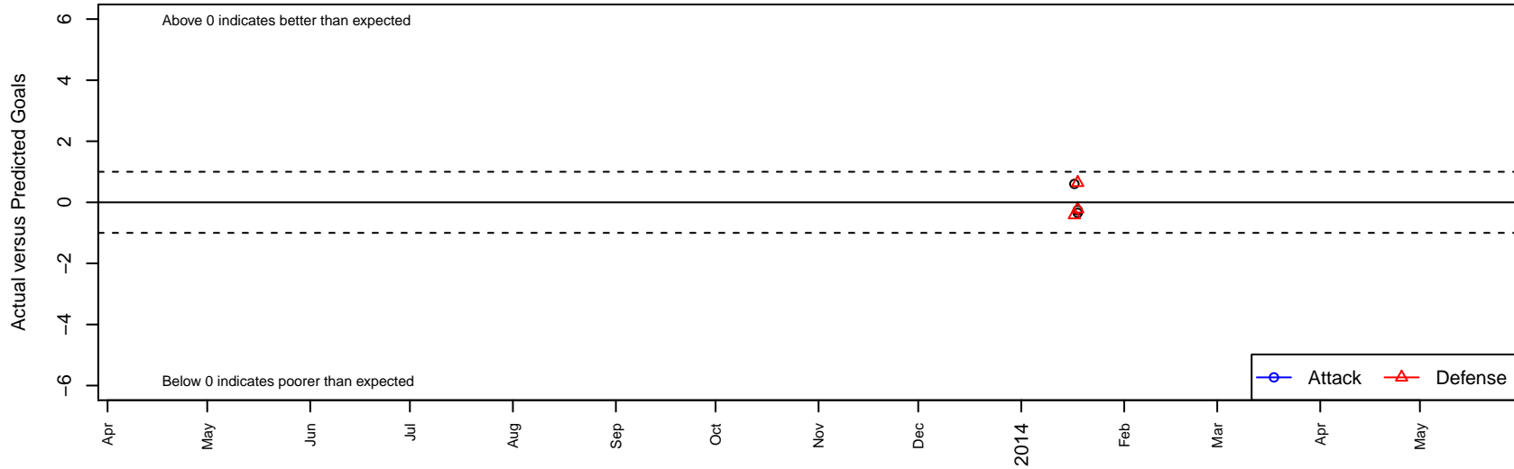
Fire FC 02 Premier B01 Dots are actual minus expected GF (blue circles) and GA (red triangles). Blue line is smoothed change in attack strength. Red is smoothed change in defense strength.
